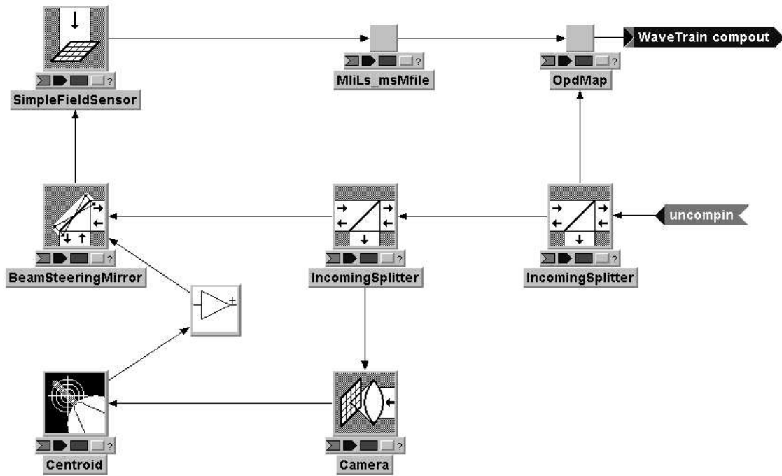
Figure 3.5. Compensator block.
